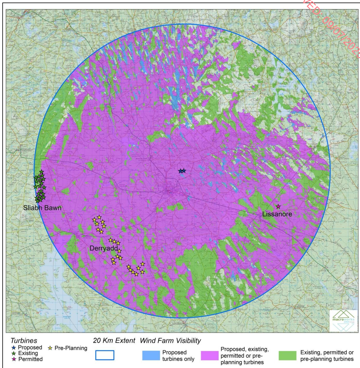
Figure 5.13 Cumulative ZTV including potential future windfarm developments
