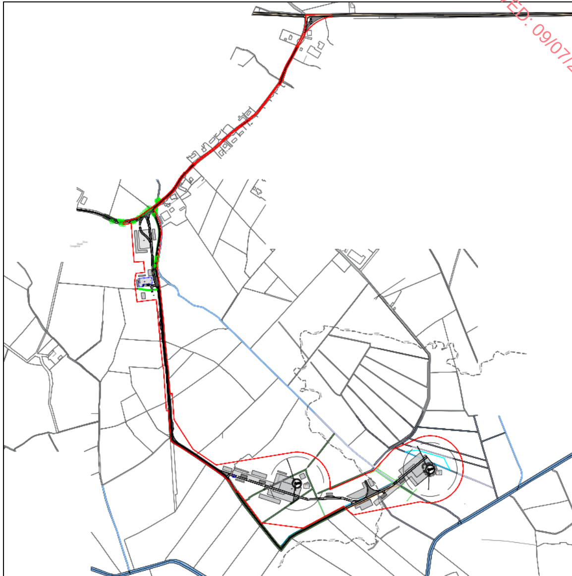
Figure 1.1 Site Layout (extract from Dwg. No. 22729-101)
