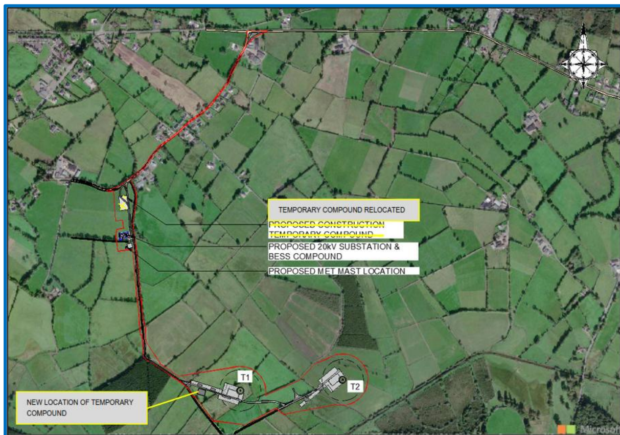
Figure 2.3 Proposed Development Layout
