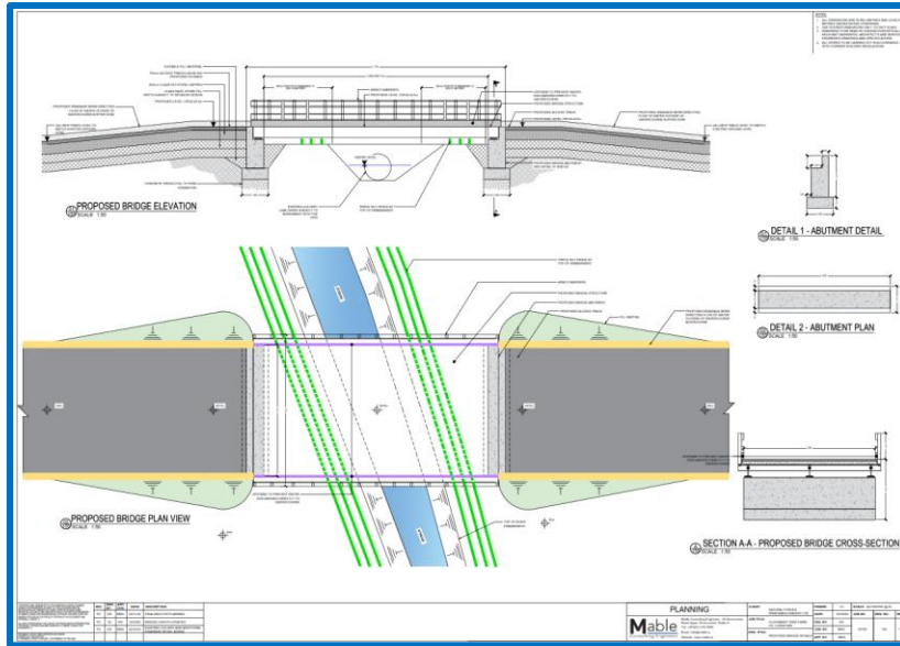
Figure 2.9 Stream Crossing – Bridge Installation
