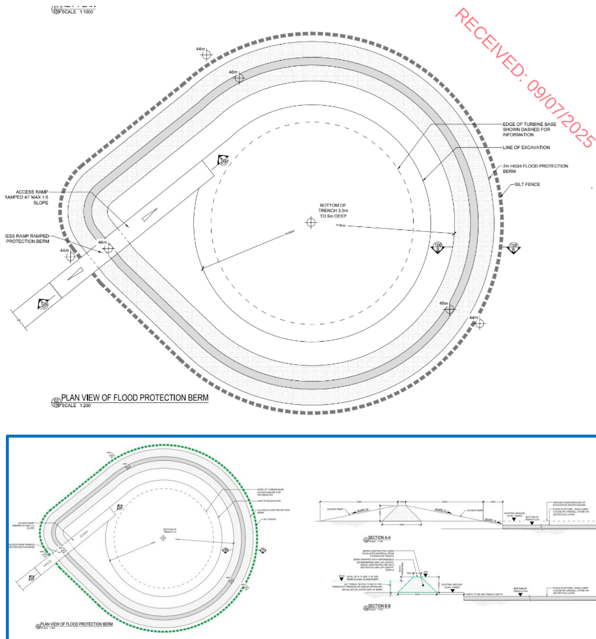
Figure 2.18 Plan view of Flood Protection Berm (Drawing 22729-156)
