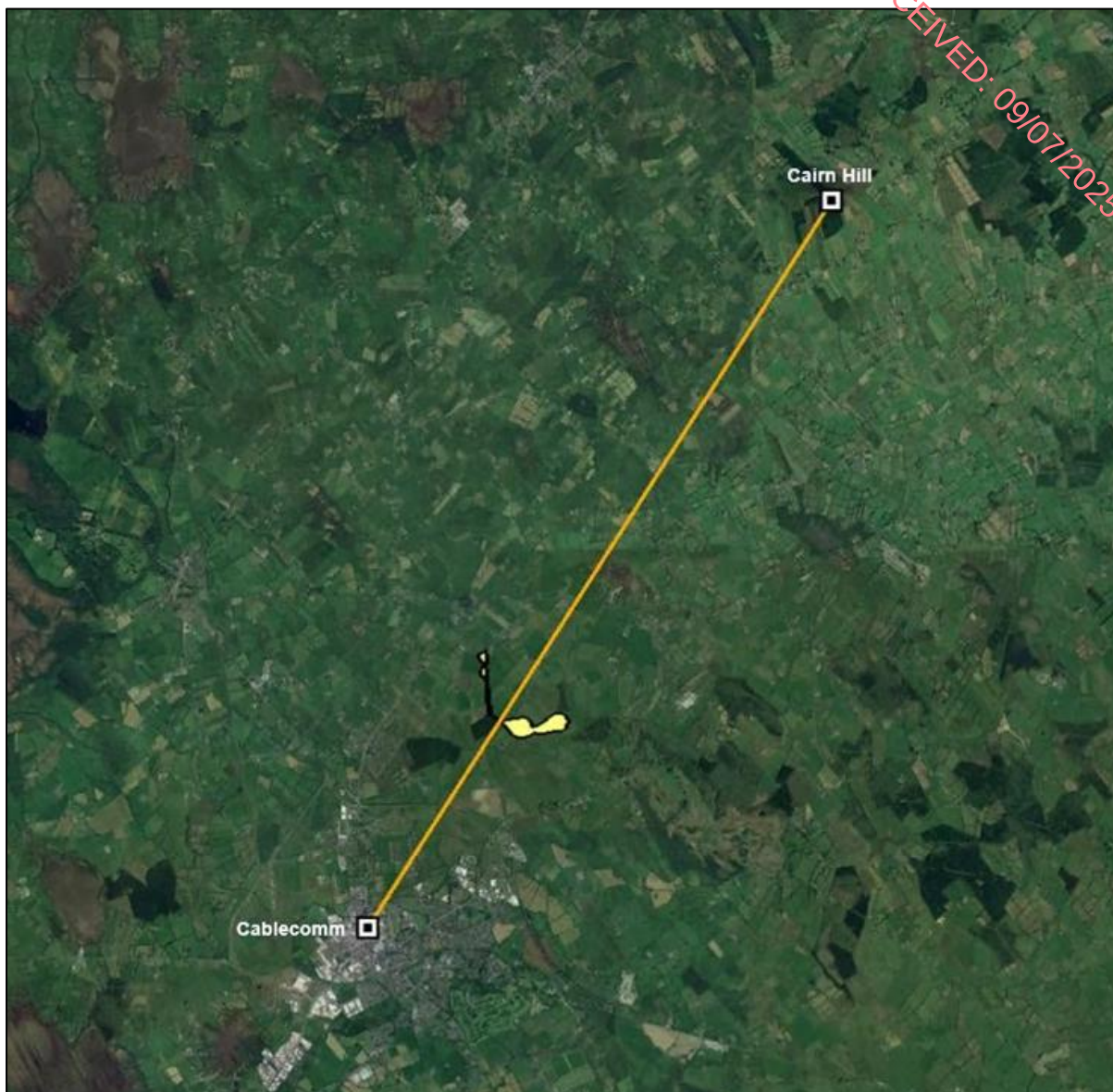
Figure 7-6 - Eir Radio Network – Plan View - Telecommunications study area outlined in yellow.
