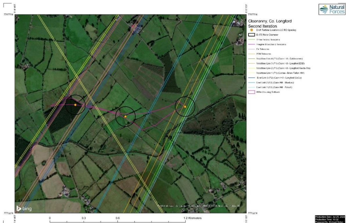
Figure 3.6 Alternative Turbine Layout 2 Showing Telecommunication Links
